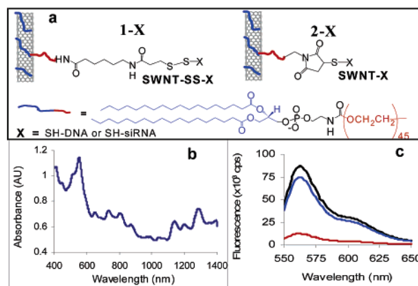
Figure 1. (a) Two schemes of SWNT functionalization by thiolated biological molecule X with ( 1-X ) and without ( 2-X ) disulfide bond respectively. Both DNA and RNA cargos contain a thiol functional group and a six-carbon long spacer at the 5' end of the DNA or RNA. (b) UV–vis–NIR of a 1-DNA solution (peak at ~550 nm due to Cy3 label on DNA) and (c) fluorescence spectra (for Cy3 label) of a 1-DNA and 2-DNA , respectively, before (black) and after DTT treatment and filtration (blue for 2-DNA and red for 1-DNA ).
